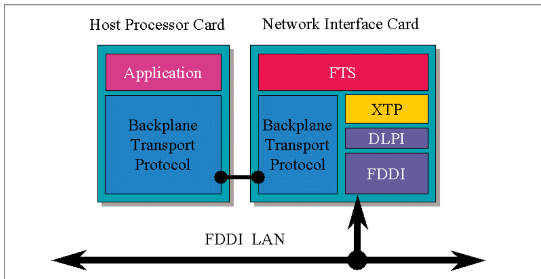
Figure 1 : XTP in the ISO OSI Protocol Stack
