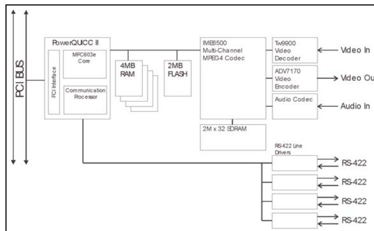
Video Capture and Compression Block Diagram
