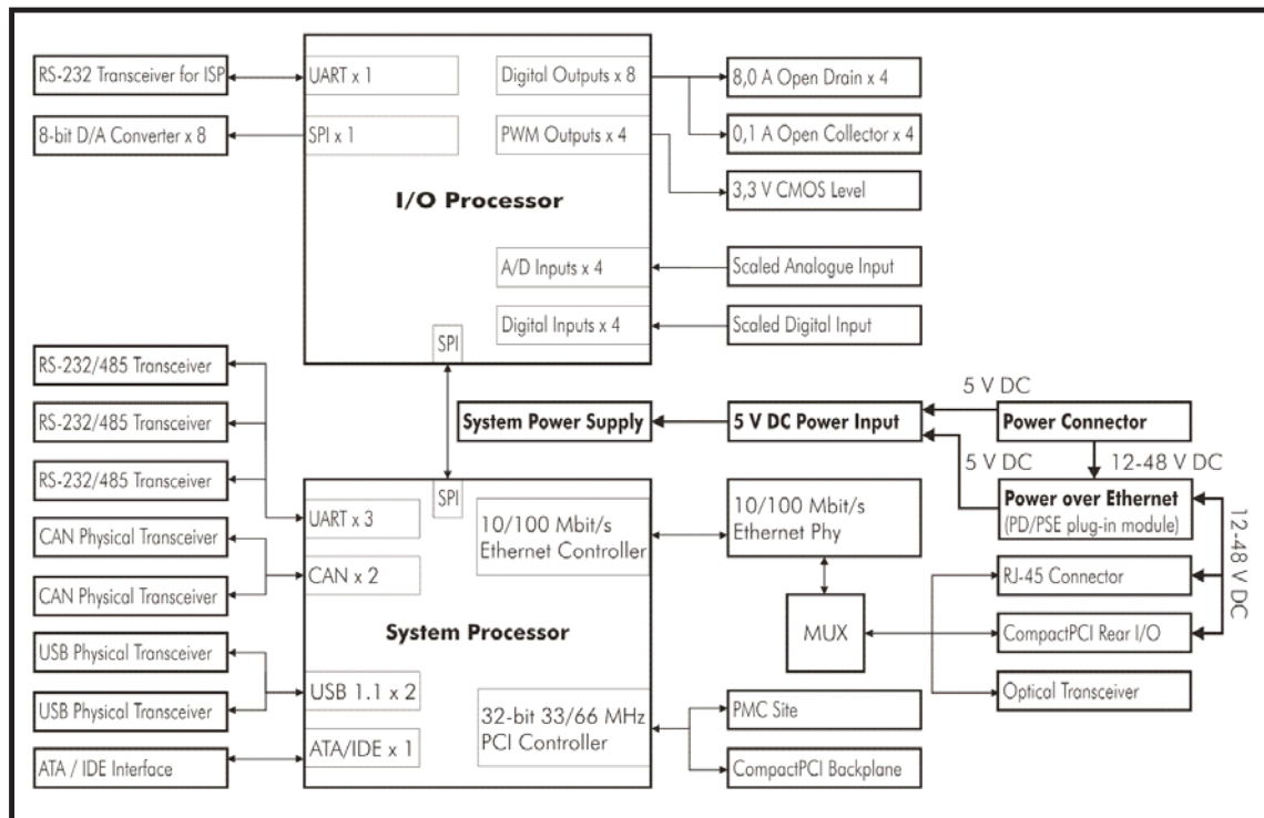
Universal Fibre Hub Functional Block Diagram
