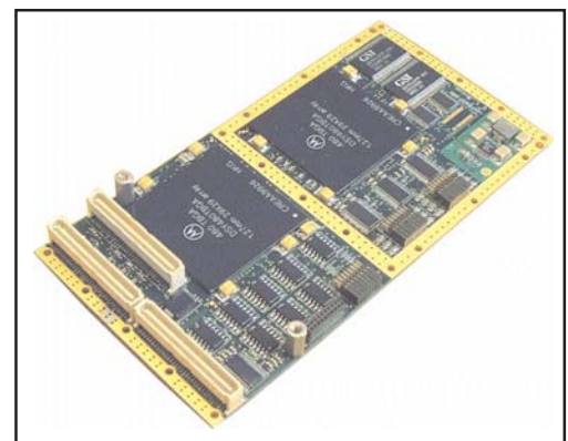
8-Channel High-Speed Serial I/O CCPMC Adapter
