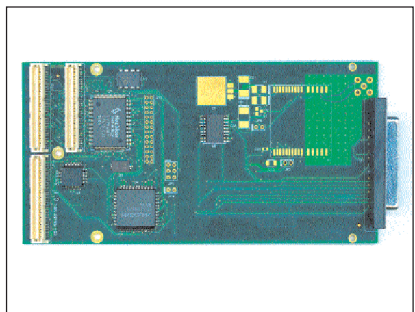
2-Channel UART Serial I/O PMC Adapter
