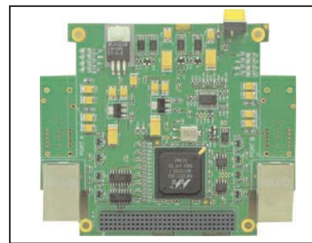
Dual Gigabit Ethernet PCI-104 : Copper Media
