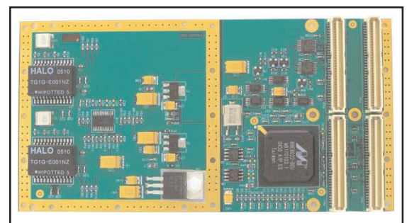
Dual Gigabit Ethernet Conduction-Cooled PMC Adapter
