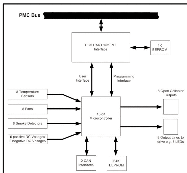
EMAC Architecture
