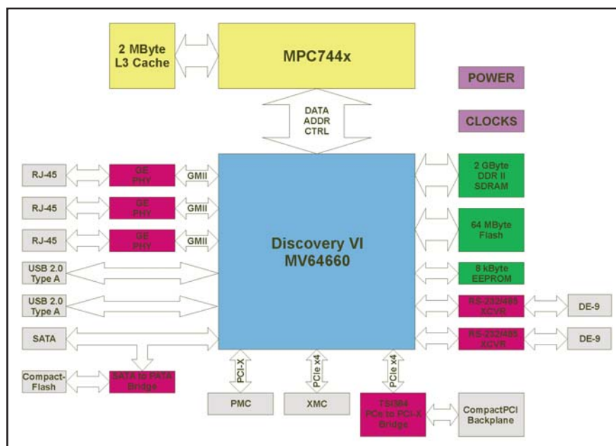
Figure 1 : MPC744x CompactPCI Host Computer Block Diagram
