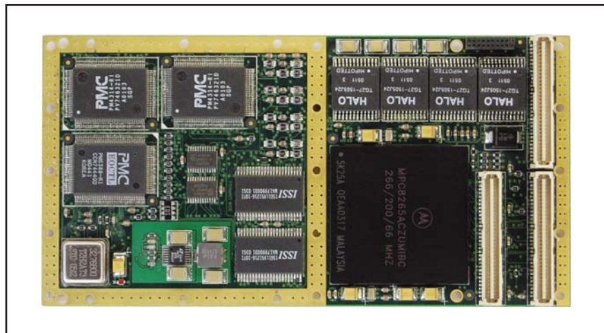
8-Channel E1/T1 Telecomms PMC Adapter
