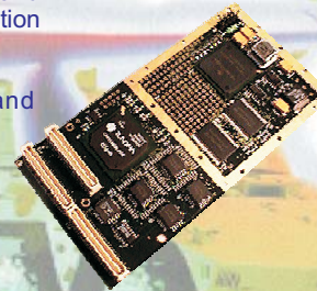
CCPMC High-Speed Serial I/O Adapter
